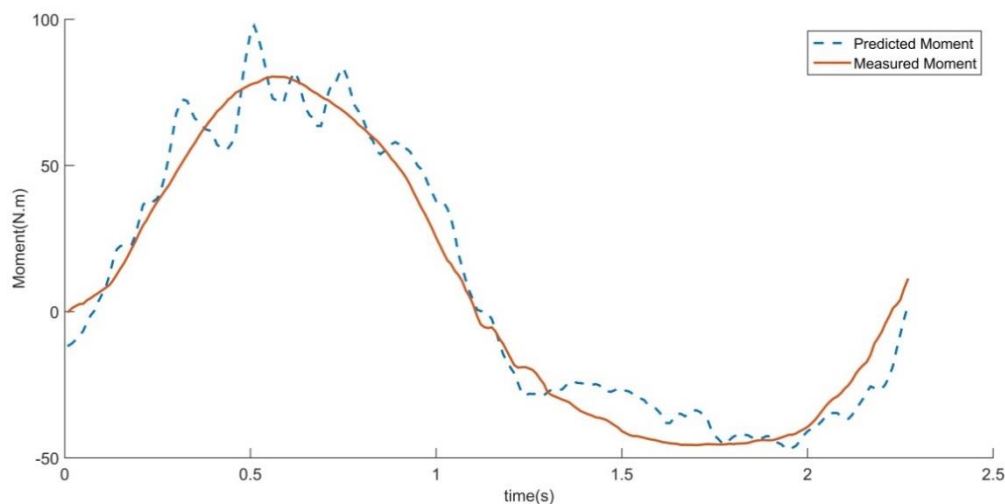
Figure 1: The moments measured and estimated by the EMG linear envelope driven model
